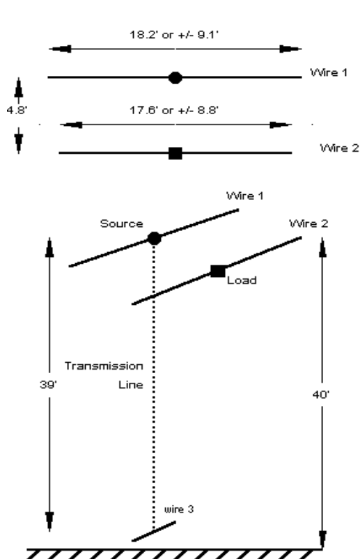
Figure 1. Antenna used as a NEC deck sample.
